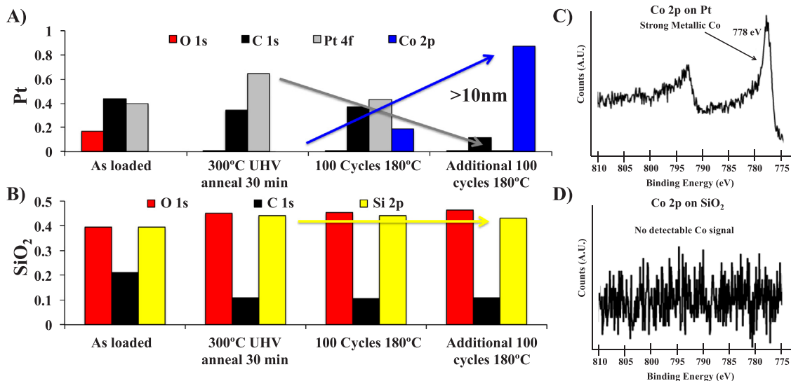
Fig. 3. XPS of UHV annealed substrates that underwent 100 + 100 additional ALD cycles of \text{Co(dad)}_2 + \text{HCOOH} at 180 °C. (A) On Pt, a completely buried Pt signal was consistent with a film > 10 nm thick. The rapid decrease in the Pt signal (grey) was consistent with a conformal film. (B) On SiO 2 , the constant Si signal and lack of a Co signal indicated no Co consistent with infinite selectivity. Raw XPS Co 2p spectra showed a strong metallic component on (C) Pt, while no observable spectra is observed on (D) SiO 2 .
