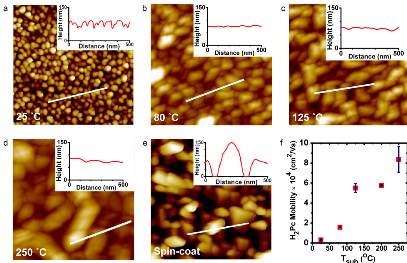
Fig. 3. \text{H}_2\text{TBP} and \text{H}_2\text{Pc} film microstructure characterization. Atomic force microscopy (AFM) images of a 1 \mu\text{m} \times 1 \mu\text{m} region of 100 nm \text{H}_2\text{Pc} deposited on \text{SiO}_2 substrates held at (a) 25 °C, (b) 80 °C, (c) 125 °C, (d) 250 °C. (e) AFM image of 1 \mu\text{m} \times 1 \mu\text{m} region of solution processed \text{H}_2\text{TBP} . The insets show line profiles of a 500 nm segment indicated by a white line in the image. The height scale on the line profiles is held constant to demonstrate the larger surface roughness for \text{H}_2\text{TBP} films. (f) Mobility of \text{H}_2\text{Pc} OTFTs with different substrate temperatures ( T_{\text{sub}} ). Some error bars are smaller than the markers.
